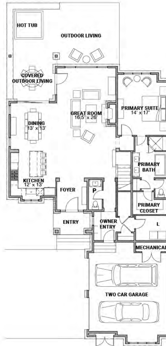
MAIN LEVEL
