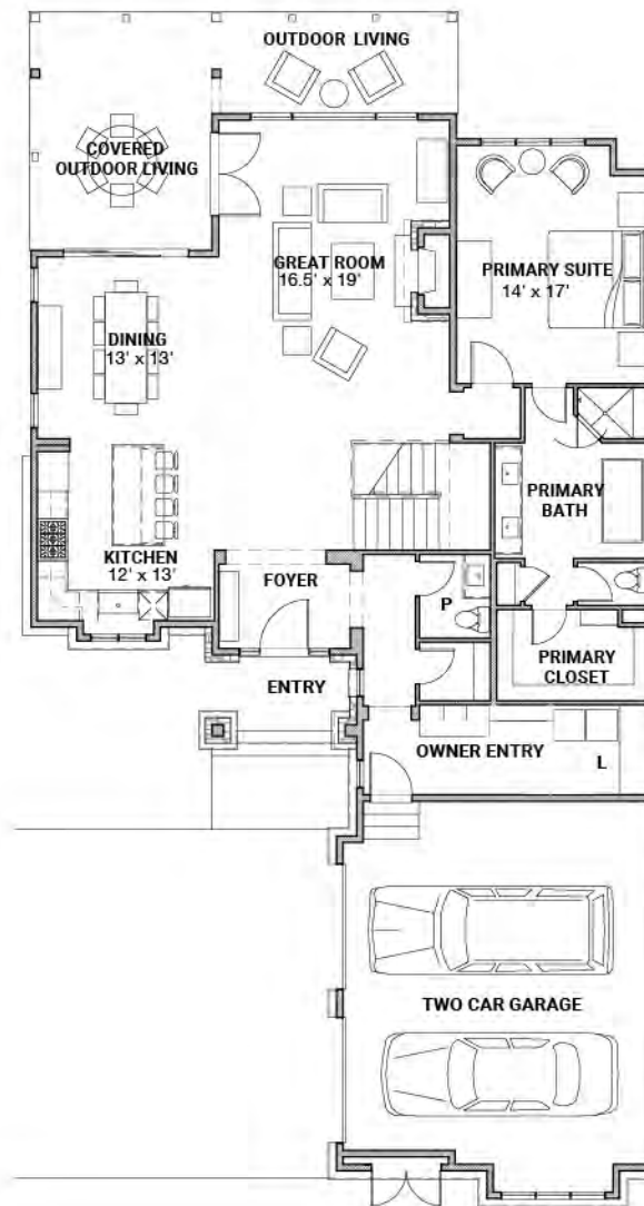
MAIN LEVEL
