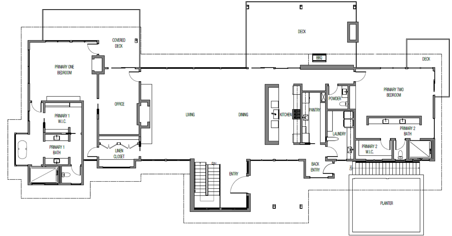
COMPOSITE LVL 2 FLOOR PLAN
